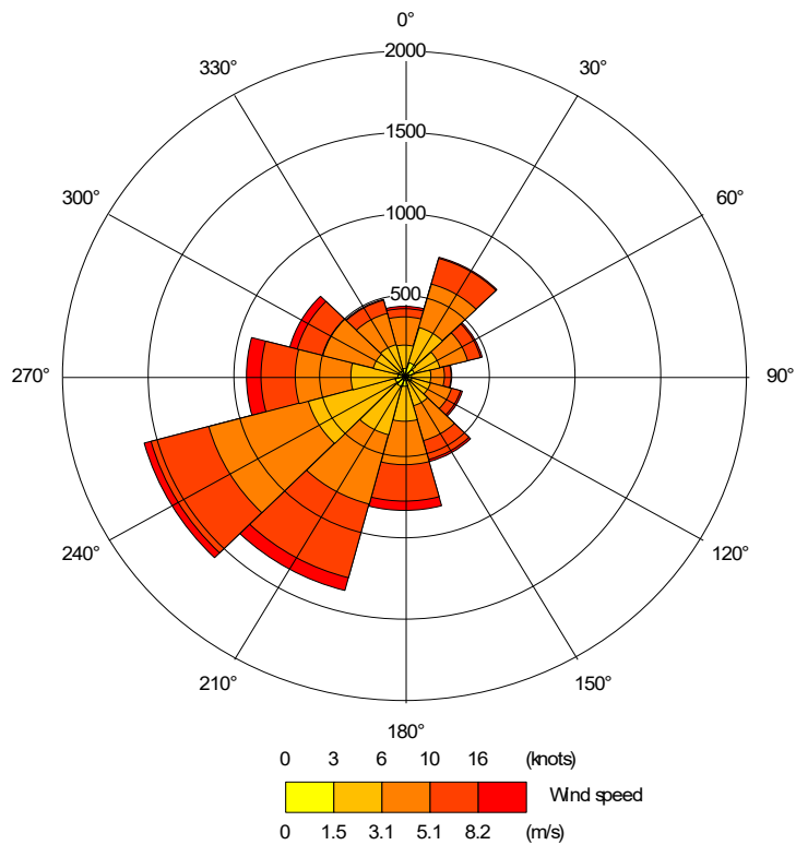
Figure 5 2022 Wind Rose for Bedford Meteorological Station
