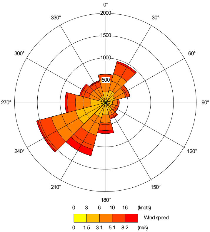
Figure 3 2020 Wind Rose for Bedford Meteorological Station
